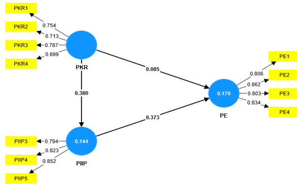
Figure 3: PLS-SEM model after bootstrapping
