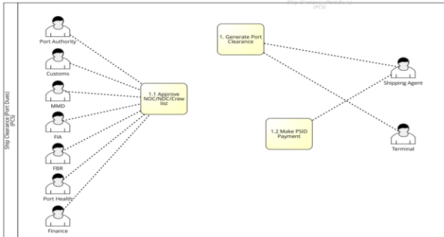
Figure 4- Proposed ship clearance process deployed via PCS-mapped on BPMN 2.0
